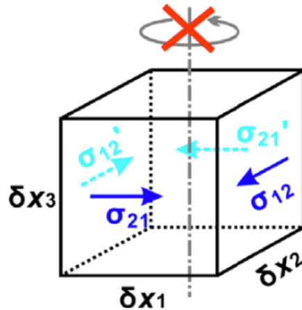
Fig. 2. The cubic prevents the rotation around x_3 axis. The blue stress tensor \sigma_{12} and \sigma_{21} must be balanced, therefore stress tensor \sigma_{12} become equal to \sigma_{21} .
